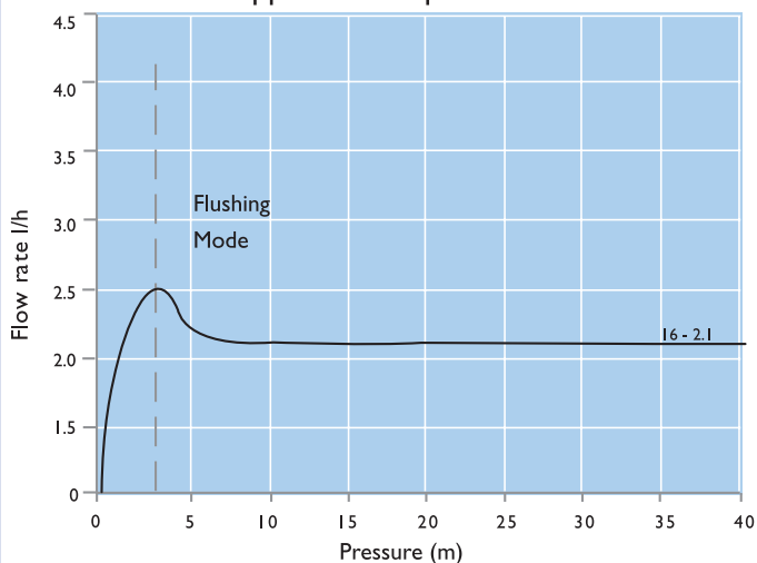
Dripper flow vs pressure
